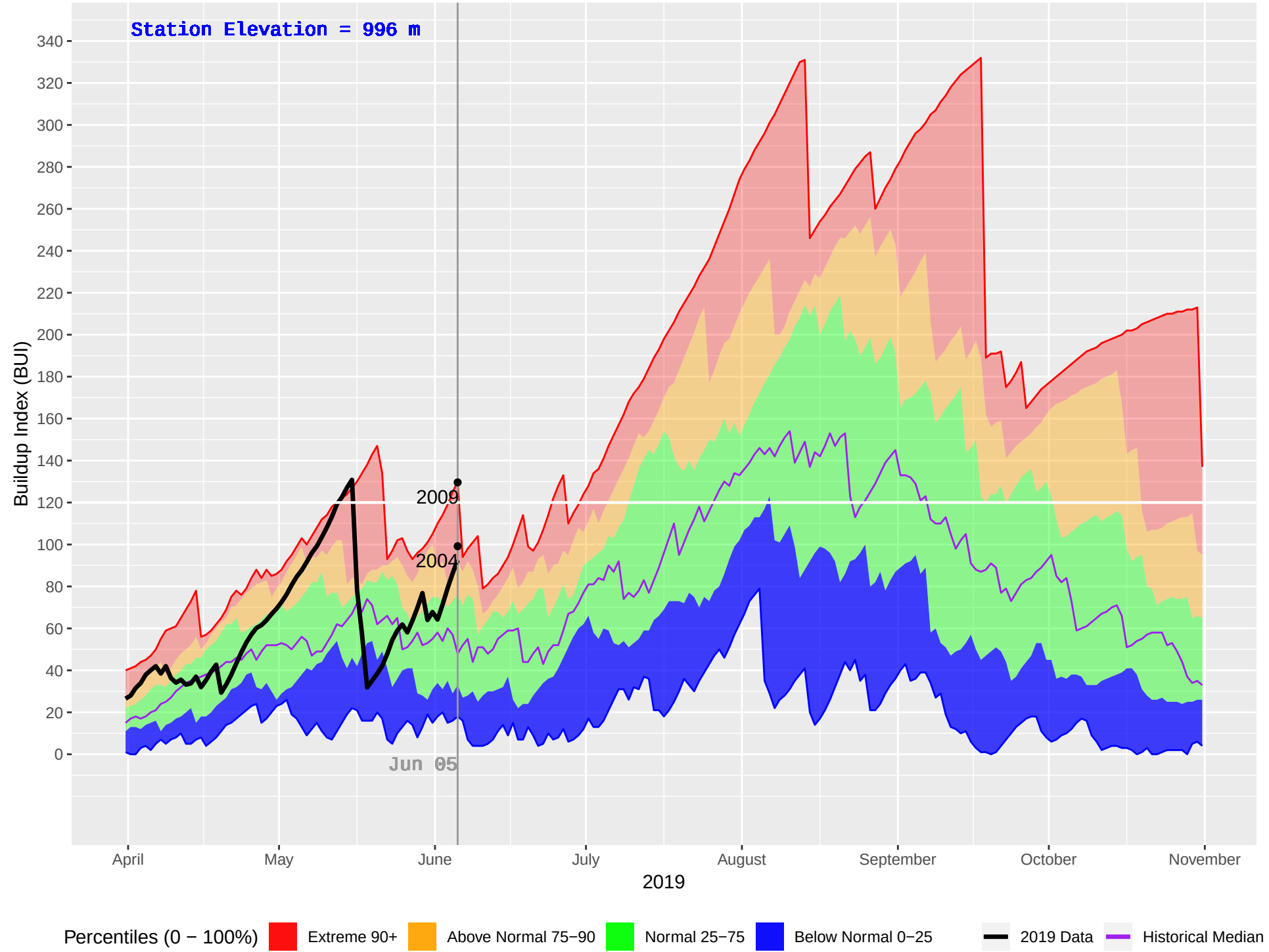
CRANBROOK FS (426) : Historical (2001–2018), Current (2019) Daily Buildup Index (BUI)
