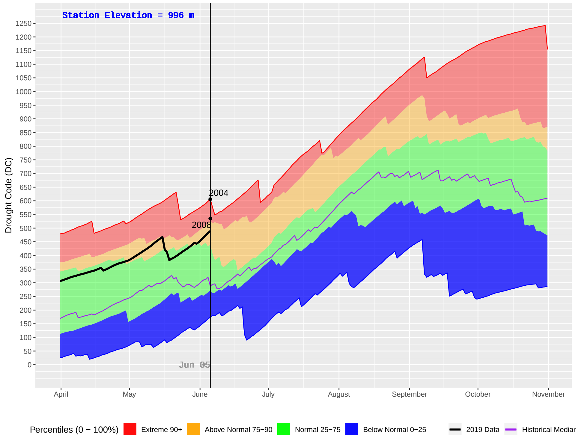
CRANBROOK FS (426) : Historical (2001–2018) and Current (2019) Daily Drought Code (DC)
