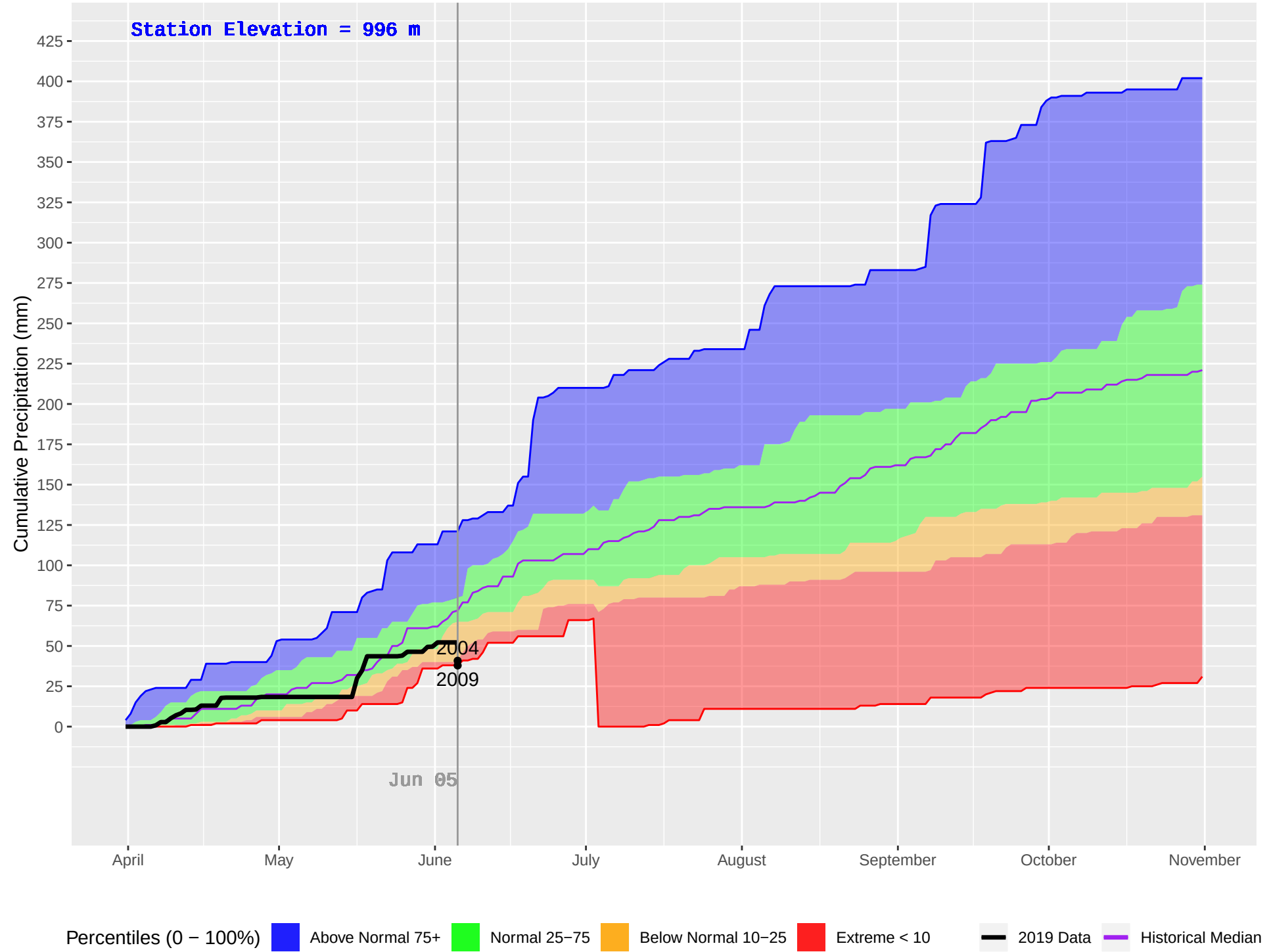
CRANBROOK FS (426) : Historical (2001–2018), Current (2019) Daily Cumulative Precipitation
