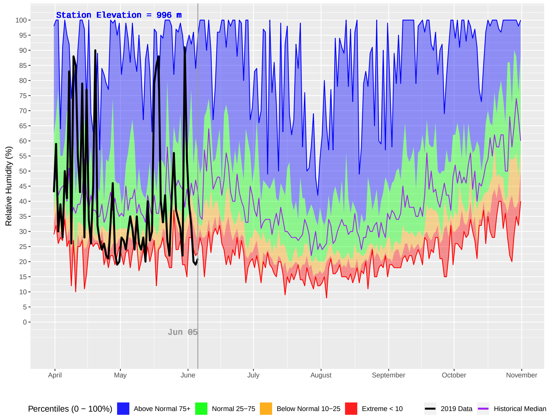
CRANBROOK FS (426) : Historical (2001–2018) and Current (2019) Daily Relative Humidity
