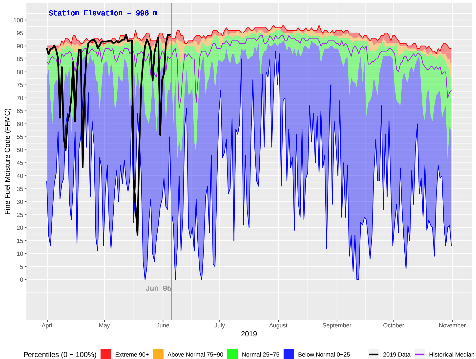
CRANBROOK FS (426) : Historical (2001–2018) and Current (2019) Daily Fine Fuel Moisture Code (FFMC)
