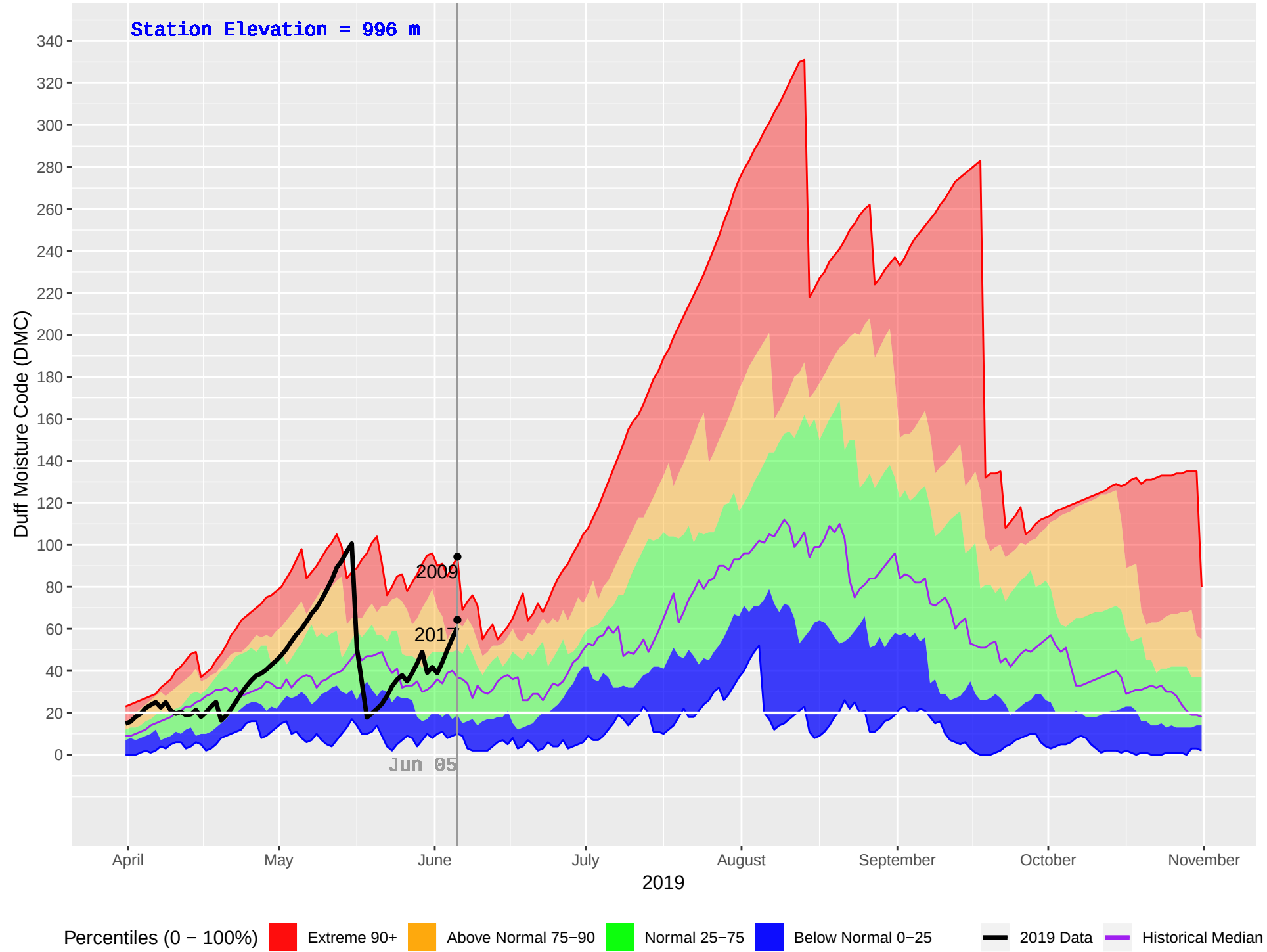
CRANBROOK FS (426) : Historical (2001–2018), Current (2019) Daily Duff Moisture Code (DMC)
